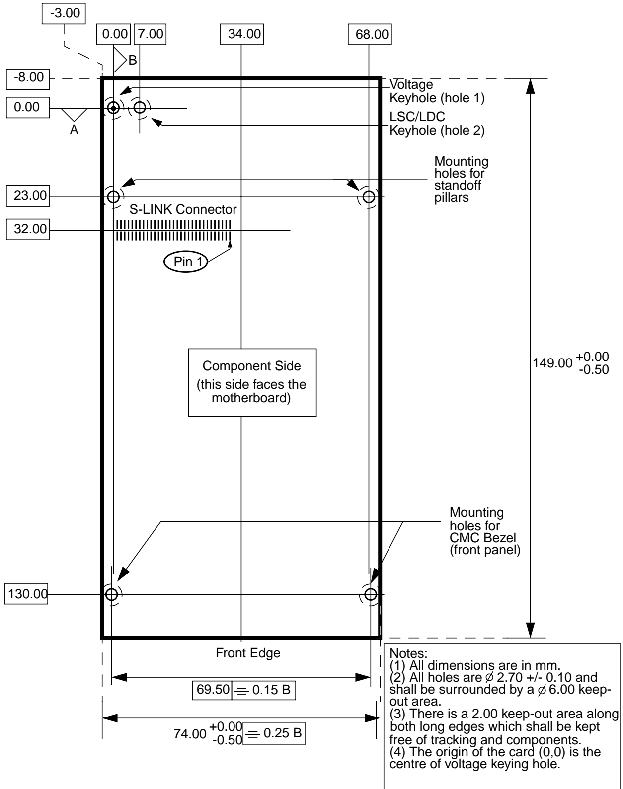
FIGURE 11. S-LINK card
