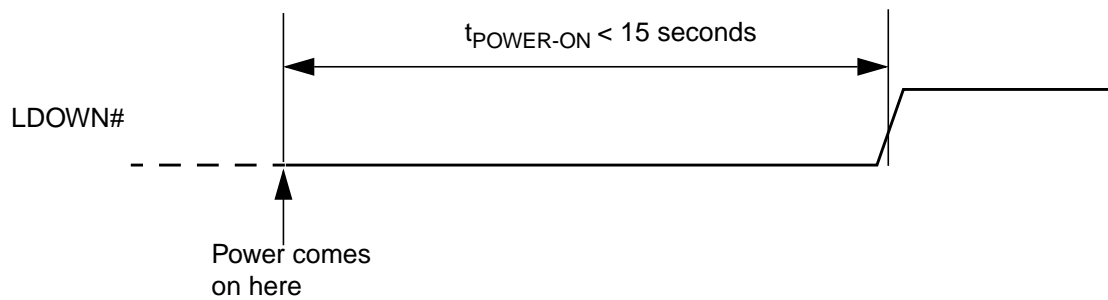
FIGURE 8. LDOWN# at Power-on
