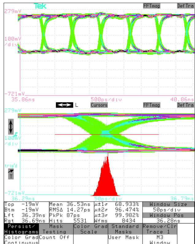
Figure 6 Eye-diagram for a 256-bit long pseudo random bit sequence at 1.2Gbit/s.
